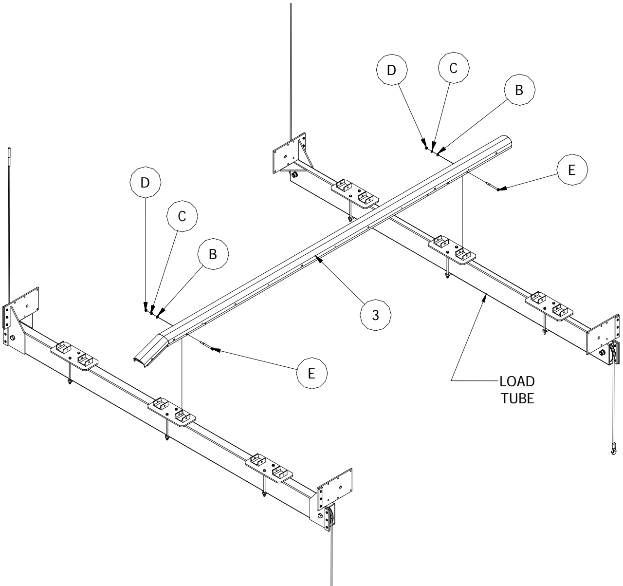
Figure 2-3.
