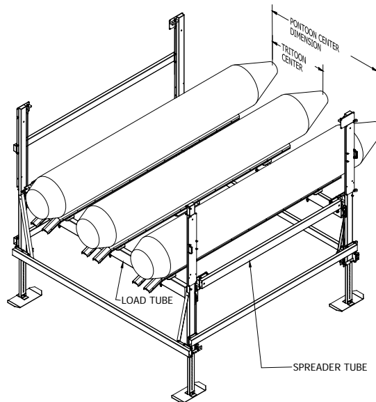
Figure 2-1. Cradle Positioning
