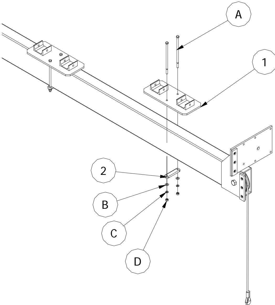
Figure 2-2. Cradle Mounting Plate Assembly
