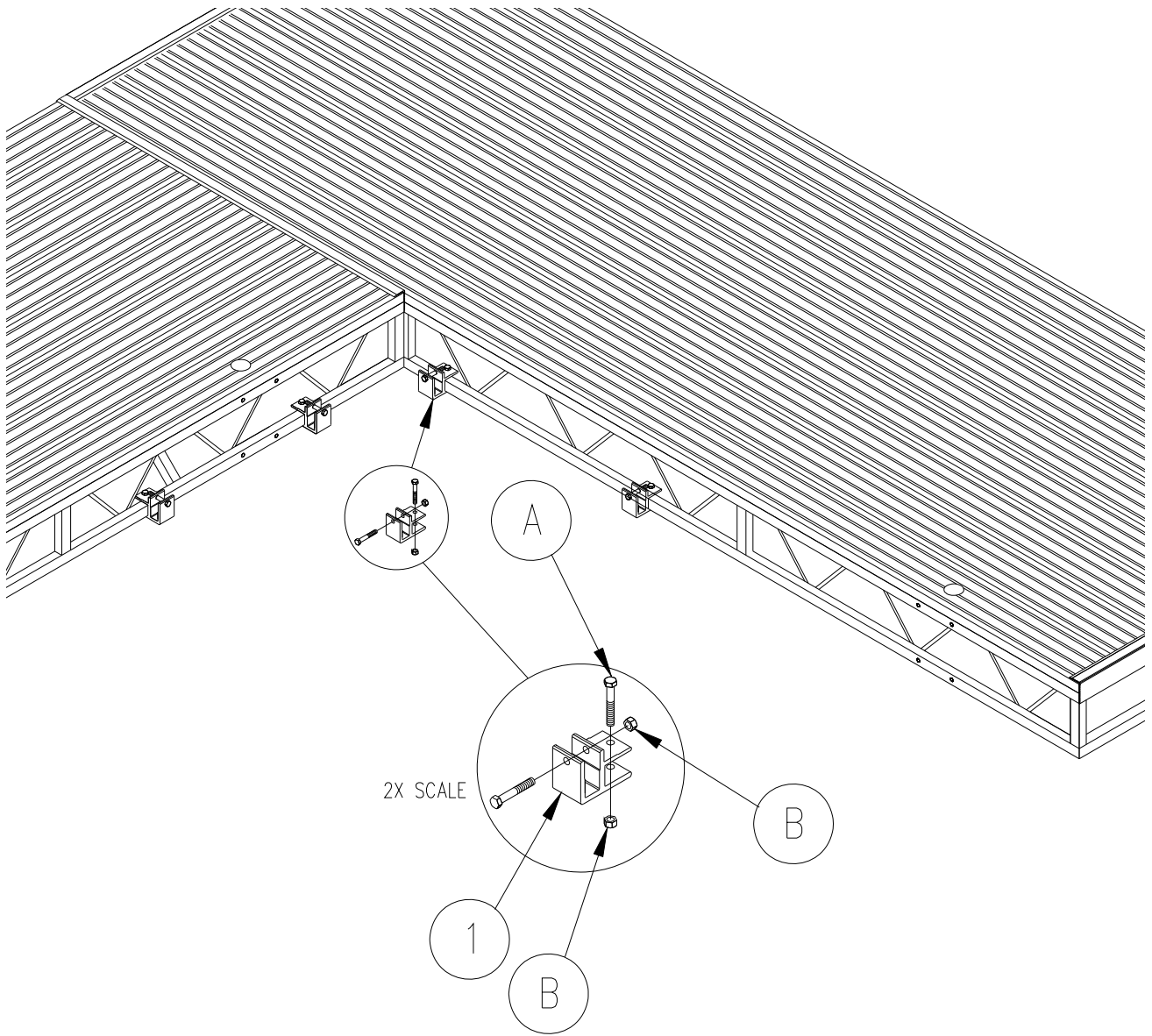
Figure 1-1 T-Dock Corner Bracket Install
