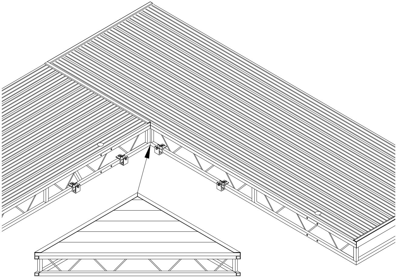
Figure 2-2 T-Dock Corner Assembly
