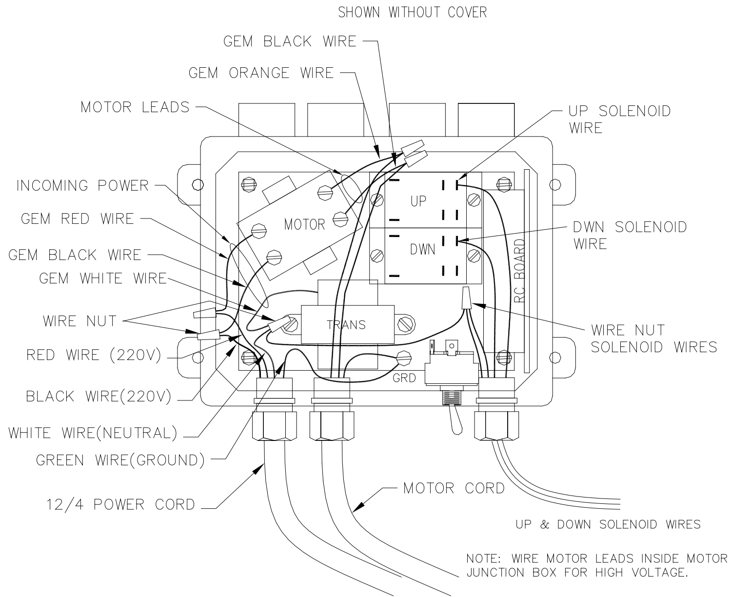
Figure 6-3 HL & HVL Power Unit 220VAC- Electrical Schematic
