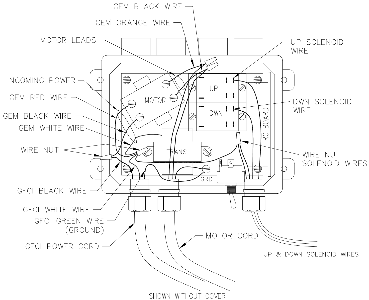
Figure 6-2 HL & HVL Power Unit 110VAC- Electrical Schematic
