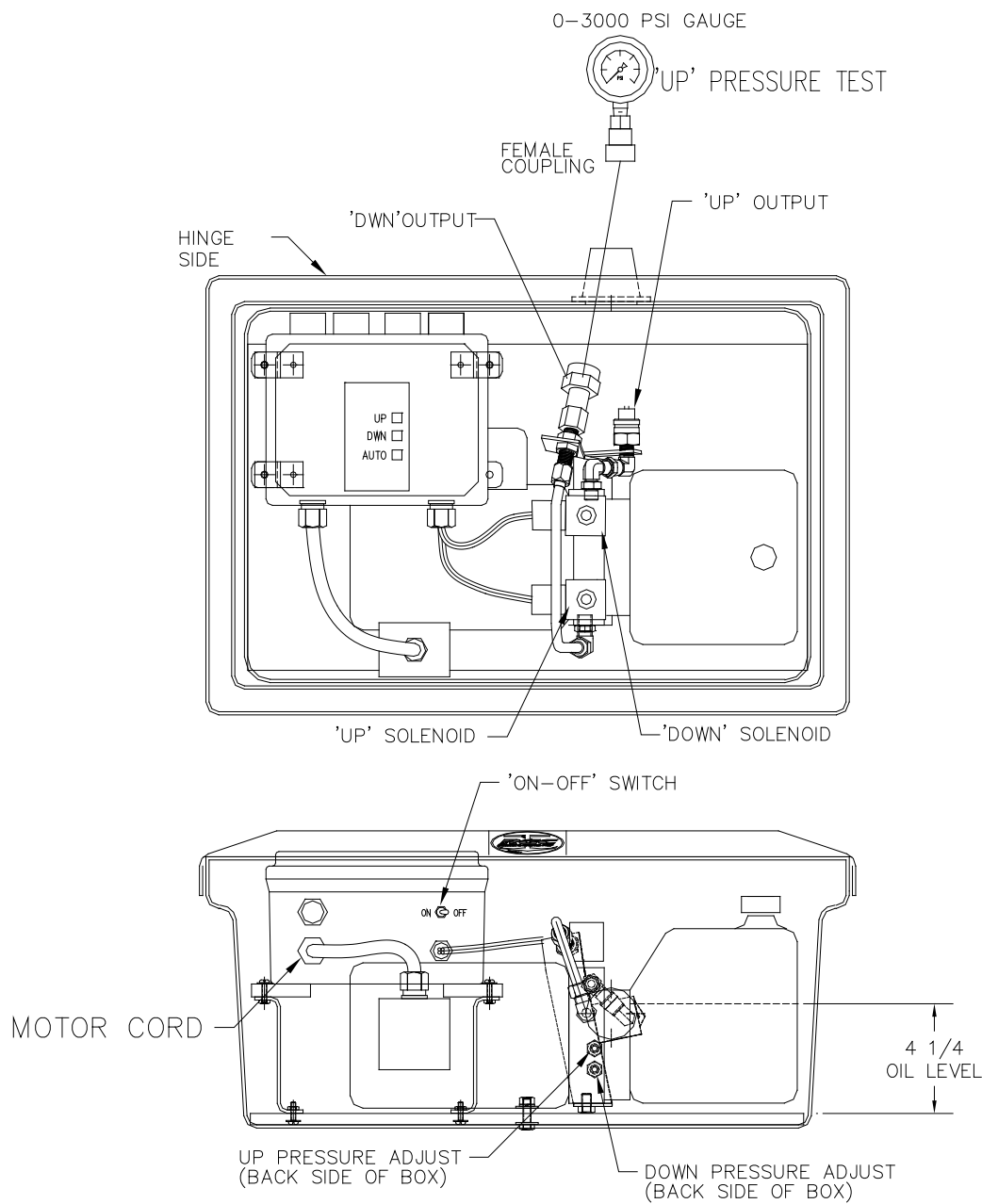
Figure 6-1 HL & HVL 120VAC Power Unit Pressure Test
