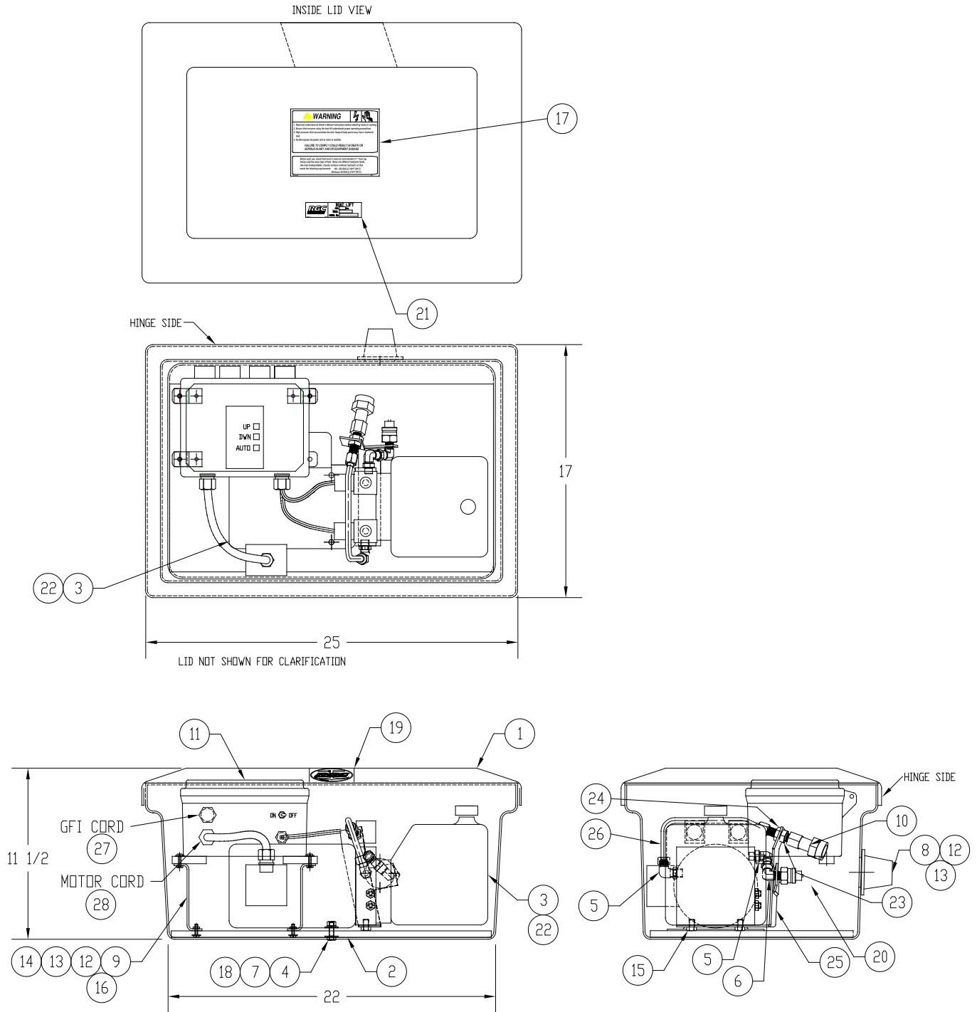
Figure 7-1 Complete HL 120/220VAC Power Unit Assembly
